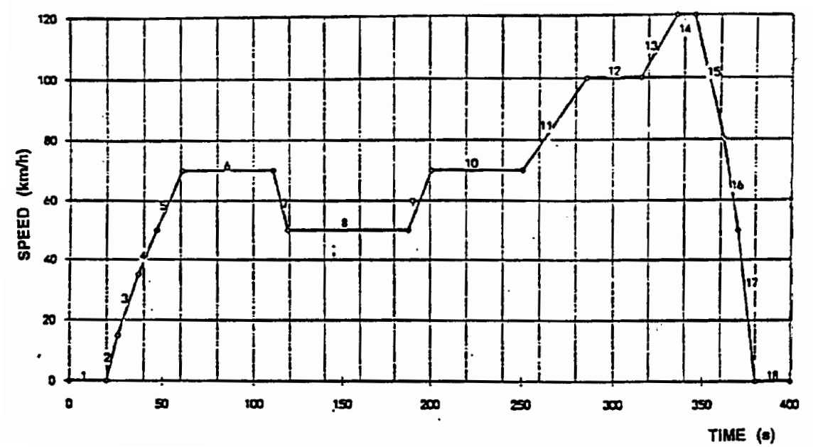
Figure 3 Extra-urban cycle (400 seconds)
