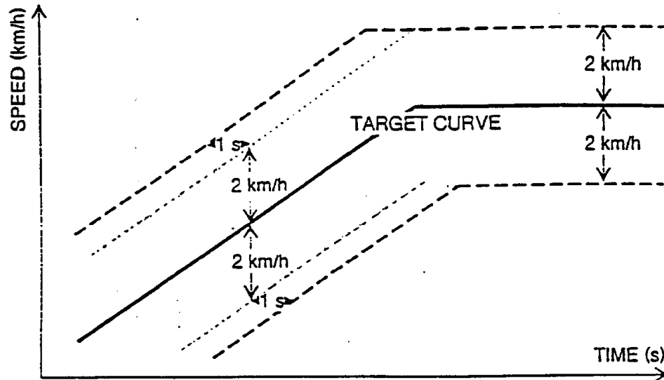
Figure 4 Speed tolerance
